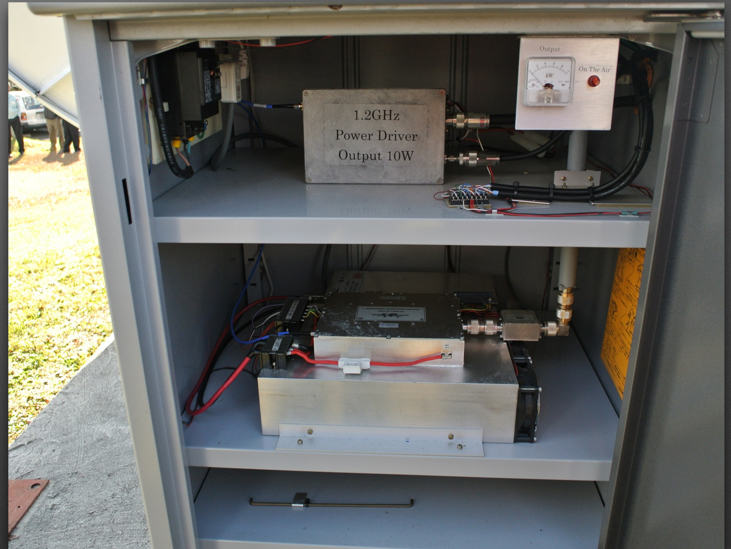
1.2GHz 500W Linear Amplifier
